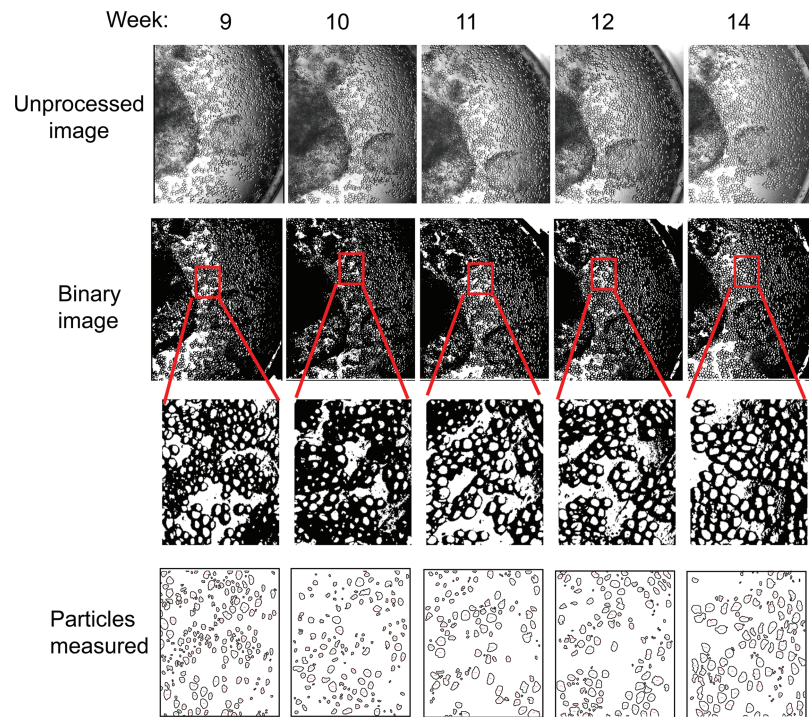
SUPPLEMENTARY FIG. S1. Quantification of adipocyte size in explant cultures. Brightfield images of explants in 96-well multiwells were obtained using a 5\times objective at the time points indicated. Images were imported into FIJI, converted to eight-bit grayscale (unprocessed images), binarized (binary image), and processed as described in Materials and Methods. Most adipocytes were captured by this method, and their area recorded.
