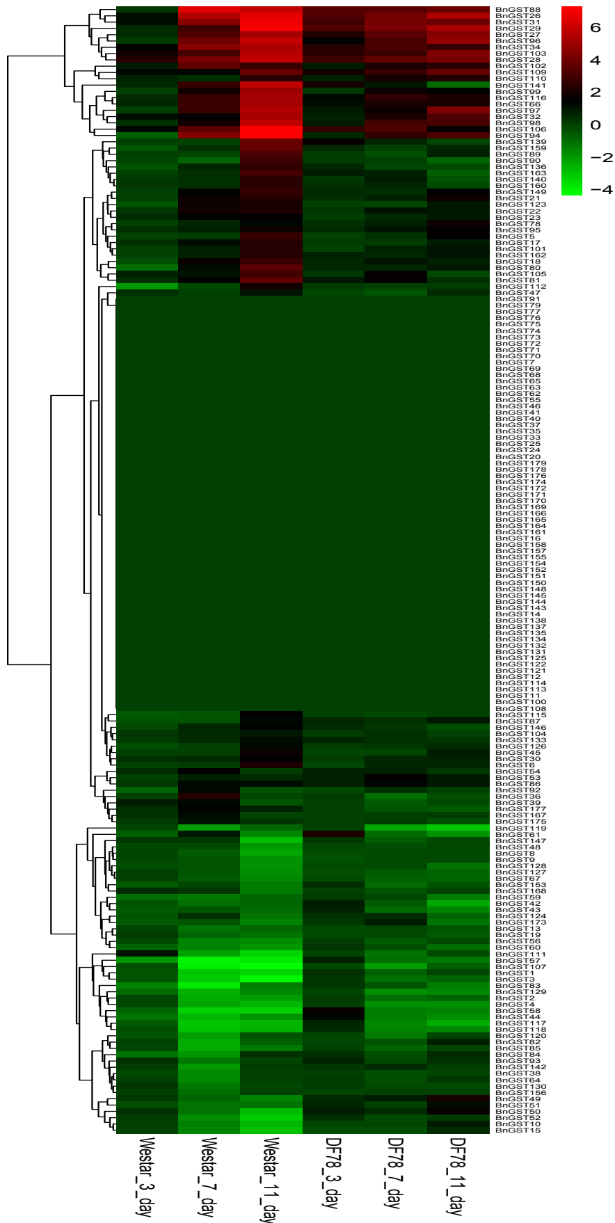
Supplementary Figure 3 Expression patterns of BnGSTs in response to Leptosphaeria maculans in B. napus .
