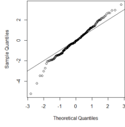
B Normal Q-Q Plot
