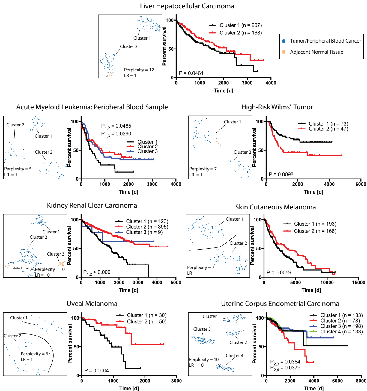
S10 Fig. t-SNE analysis of FAO-related transcripts identifies distinct tumor cohorts that correlate with patient survival. t-SNE for the FAO transcripts depicted in S2B&C Fig were analyzed in TCGA tumor types. Kaplan-Meier survival curves were then plotted for each of the clusters where significant survival differences for the indicated tumor type were observed.
