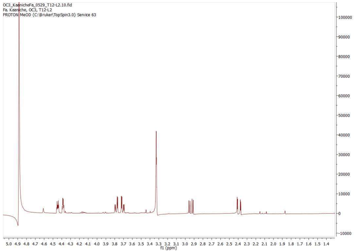
S1 Fig. ^1\text{H} NMR spectrum ( \text{CD}_3\text{OD} , 500 MHz) of 2'-deoxyribolactone ( 1 )
