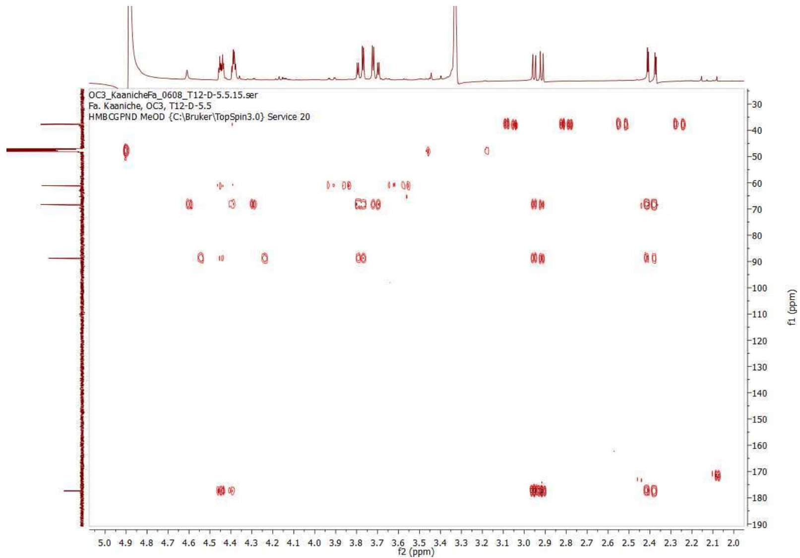
S6 Fig. HMBC spectrum (CD 3 OD, 500 MHz) of 2'-deoxyribolactone (1)
