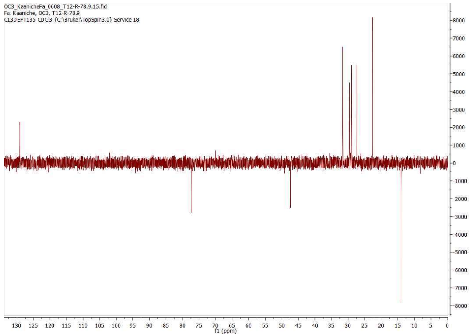
S9 Fig. DEPT spectrum (CDCl 3 , 125MHz) of Hexylitaconic acid (2)
