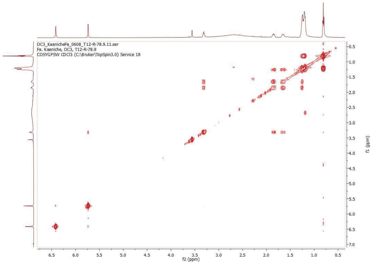
S10 Fig. H,H-COSY spectrum (CDCl 3 , 500 MHz) of Hexylitaconic acid ( 2 )
