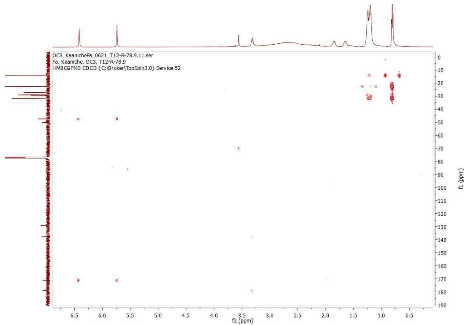
S12 Fig. HMBC spectrum (CDCl 3 , 500 MHz) of Hexylitaconic acid (2)
