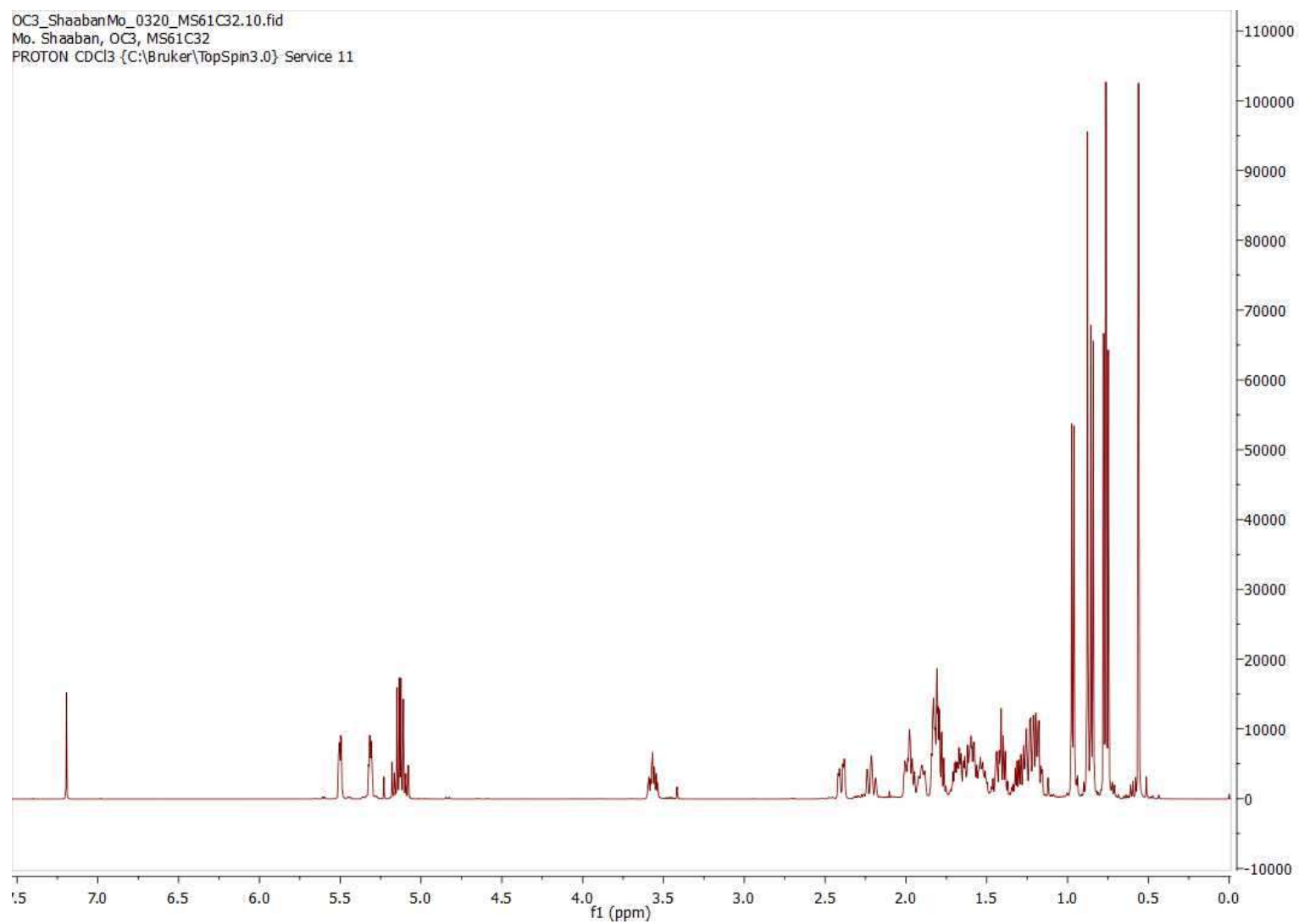
S13 Fig. ^1\text{H} NMR spectrum ( \text{CDCl}_3 , 500 MHz) of ergosterol ( 3 )
