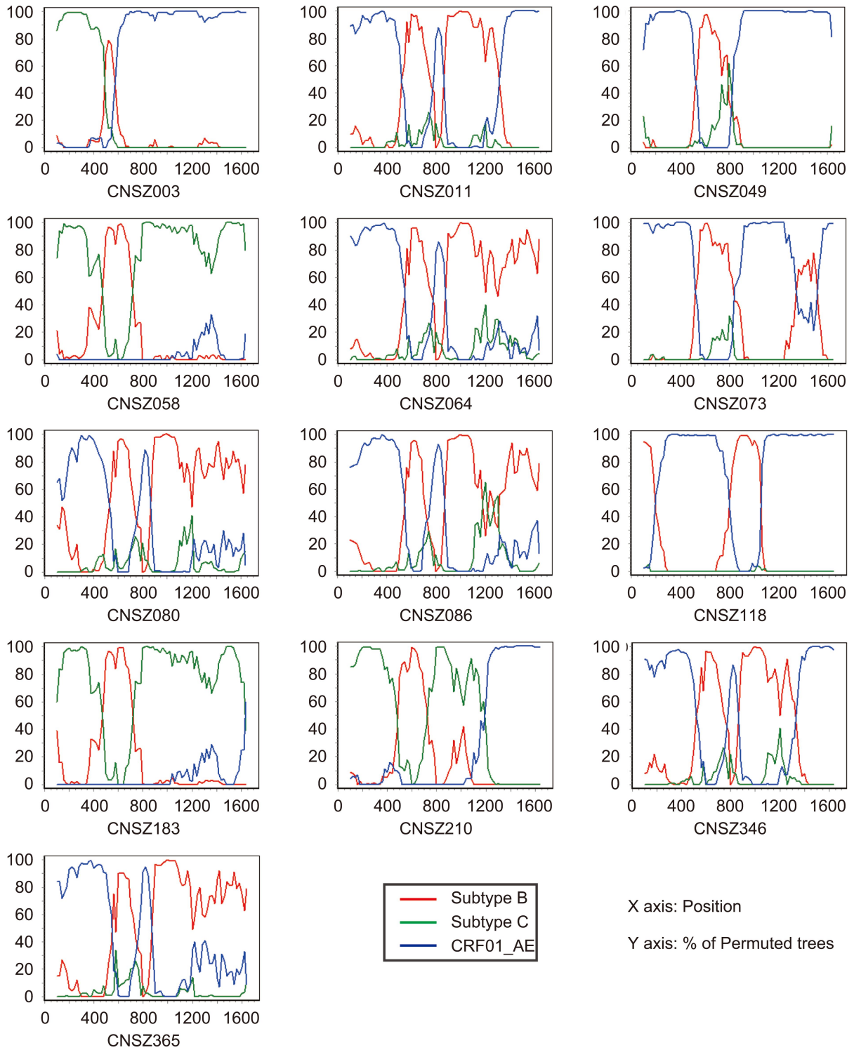
Figure S1. Recombination breakpoint analysis of the 13 URFs. Bootscan plot of percentage permuted trees over nucleotide position across the lengths of RT sequences.
