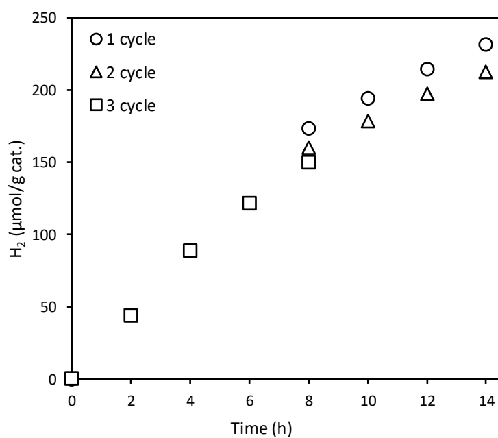
Figure S2. Production of hydrogen during the photocatalytic reduction of CO 2 in presence \alpha -Fe 2 O 3 _500 in the three cycles.
