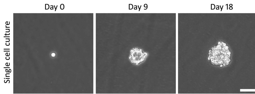
SUPPLEMENTARY FIG. S2. Single-cell culture of the ACT-derived cells. Phase contrast microscope images show a single cell that was dissociated from ACTs can proliferate and form a spherical structure at day 9. The cell sphere becomes larger at day 18. Scale bar: 50 \mu\text{m} . ACT, auditory cortex tissue.
