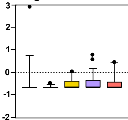
agmatine
