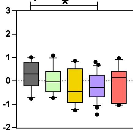
spermine
