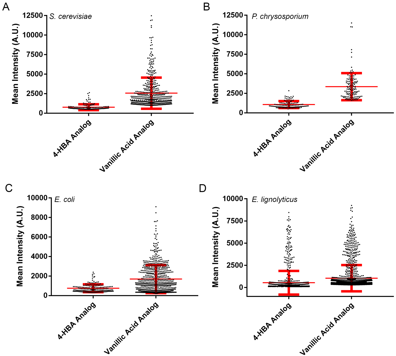
Fig. S5. Single cell Alexa Fluor™ 647 intensities of A. S. cerevisiae B. P. chrysosporium , C. E. coli , and D. E. lignolyticus . Thin red line is the mean and red whiskers mark the standard deviation. Intensities shown are from the cells deemed positive in three biological replicates based on stringent thresholds to minimize the moderate levels of autofluorescence (see Methods for detailed description). Mean intensity data is presented raw and does not compensate for the vanillic acid analog being difunctionalized.
