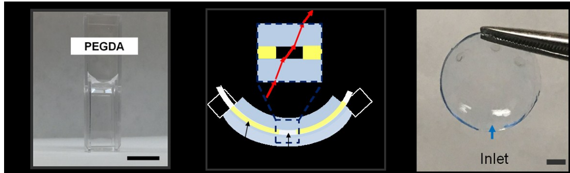
Figure S1. Evaluation of transparency of the fabricated microfluidic contact lens. (a) A photograph of the polymerized PEGDA hydrogel. Scale bar=1 cm. (b) Schematic of microfluidic contact lens cross-section. Red arrows show light propagation through the microfluidic contact lens. (c) Top view of microfluidic contact lens. Scale bar= 3 mm.
