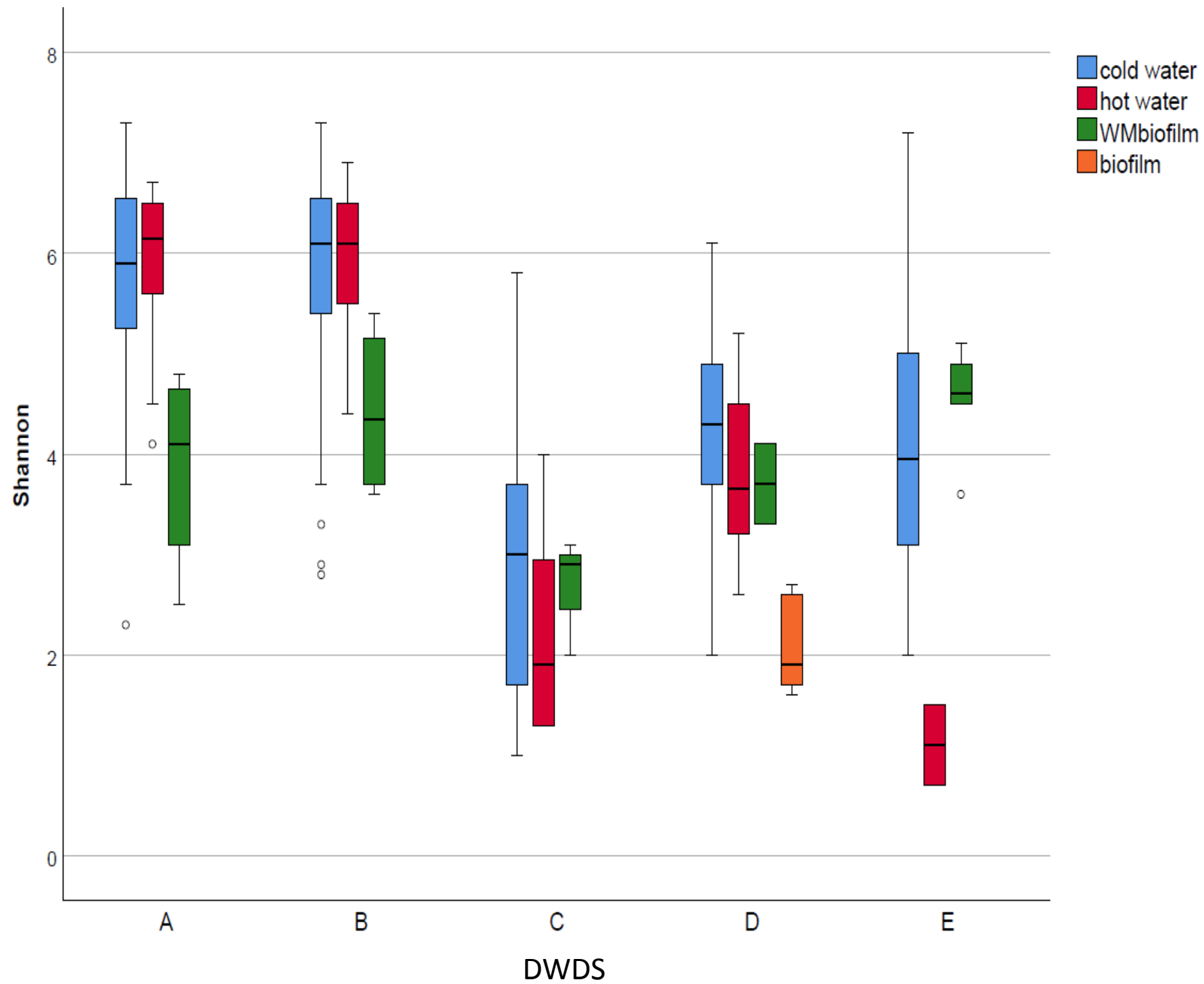
Fig. S2. Boxplot of alpha-diversity Shannon values grouped by cold water, hot water and biofilms in each DWDS A–E (DNA + RNA). WMbiofilm = water meter biofilm, biofilm = pipeline biofilm.
