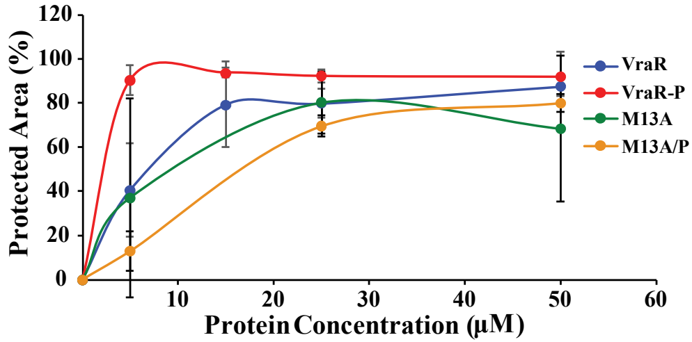
Fig. S2 Binding isotherms of VraR, VraR-P, VraRM13A and acetyl-phosphate-treated VraRM13A (VraRM13A/P). Three DNA bands from the DNase I footprinting gel, located in the VraR-protected region were used to assess VraR binding to DNA. ImageJ was used to quantify the DNA bands.
