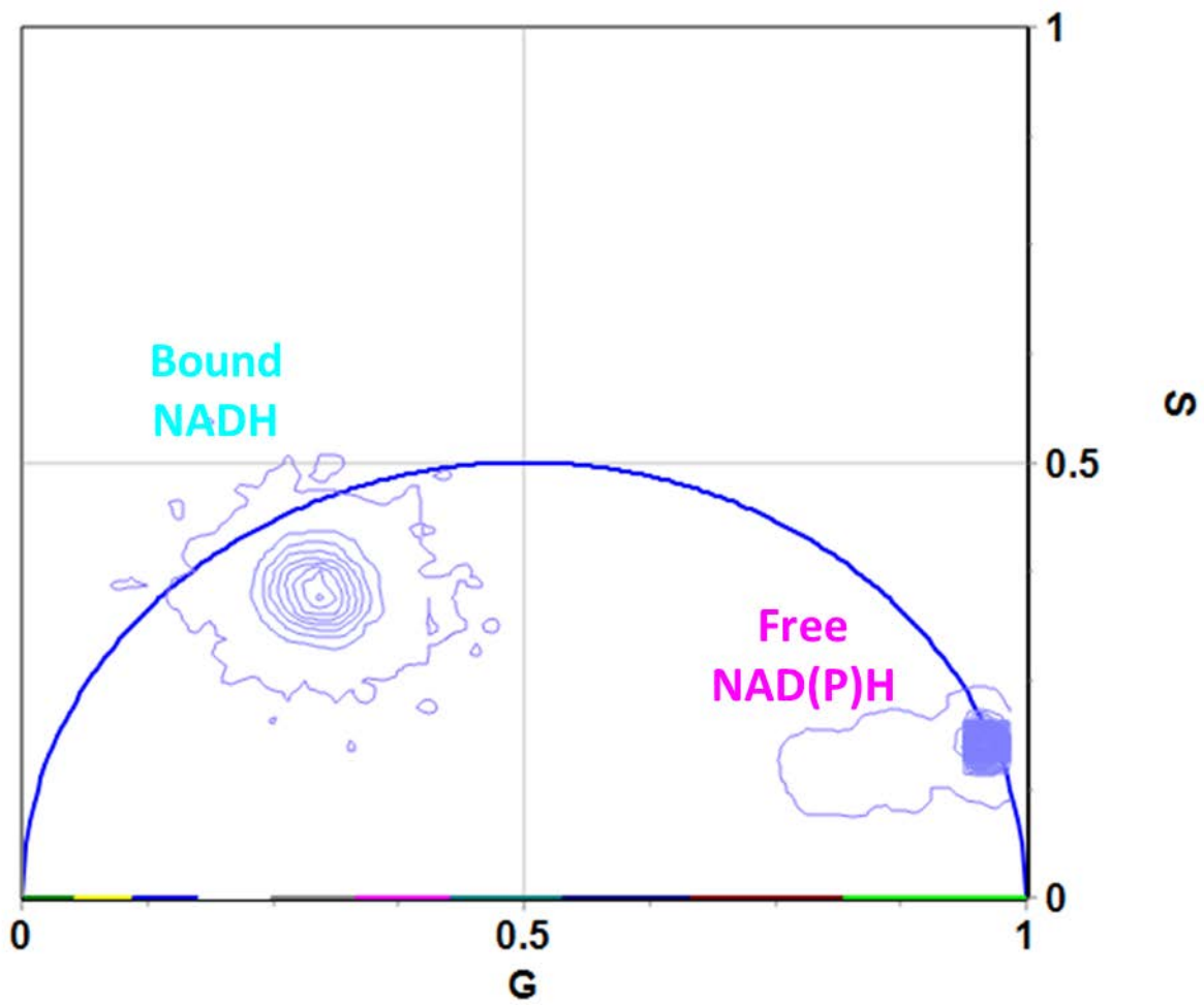
Supplementary Figure 2. Phasors of pure chemical species identify tissue components, free NADH and NADPH as well as bound NADH with lactate dehydrogenase.
