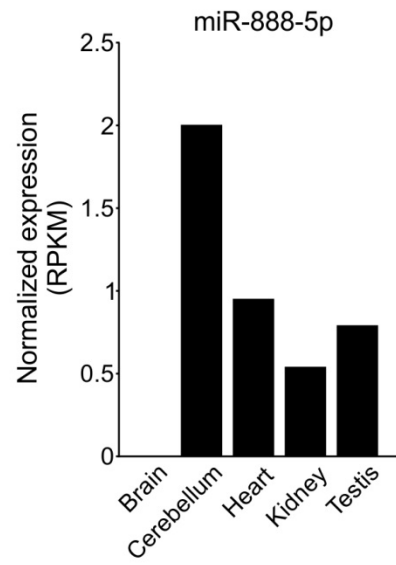
Fig. S2 Expression levels of miR-888-5p across several normal tissues. Data were obtained from MiRIAD database.
