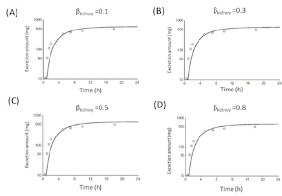
Figure S1. Simulated (lines) and observed (open circles) time profiles of metformin urinary excretion after a single oral administration of 1500 mg metformin using various \beta_{\text{kidney}} values. (A) \beta_{\text{kidney}}=0.1 , (B) \beta_{\text{kidney}}=0.3 , (C) \beta_{\text{kidney}}=0.5 , (D) \beta_{\text{kidney}}=0.8 .
