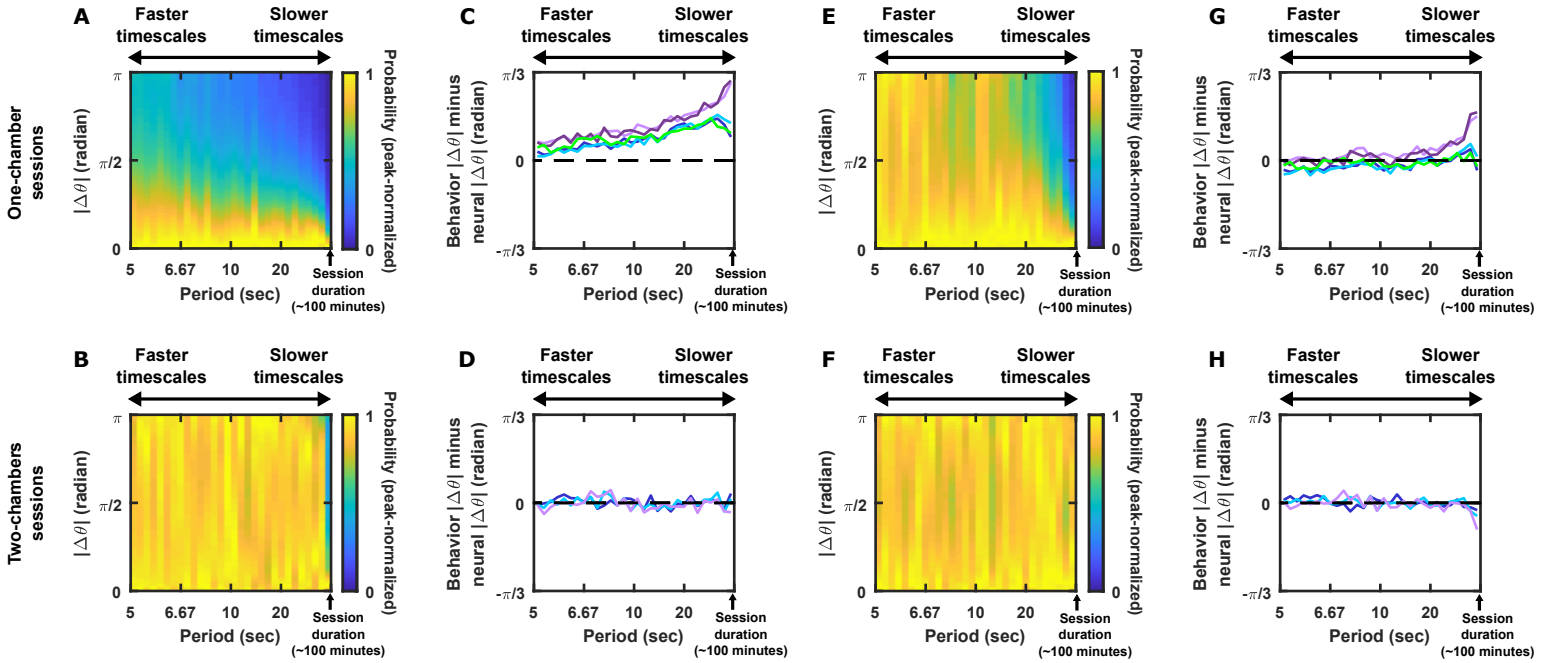
LFP, 30-150 Hz, power phase difference across bats
