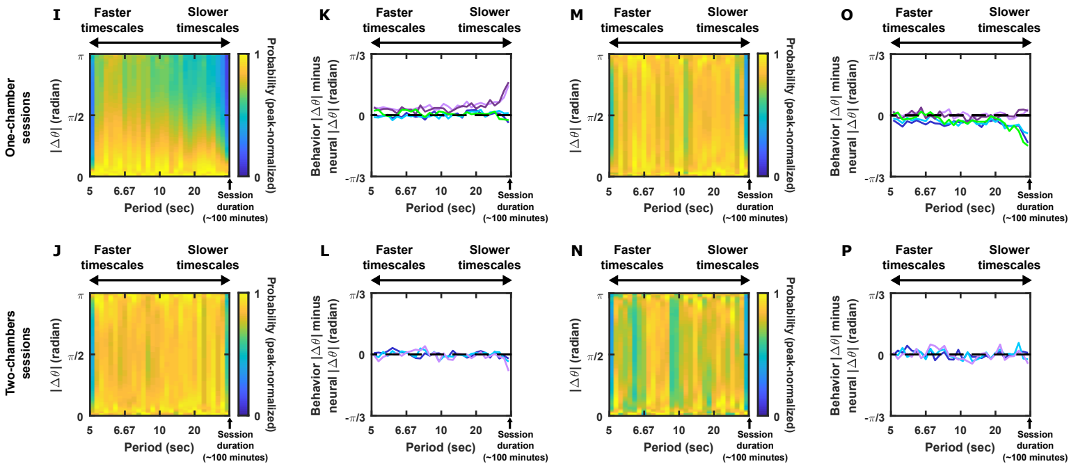
Multiunits, firing rate phase difference across bats
