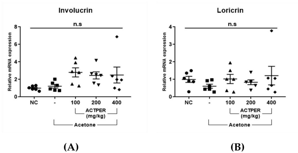
Figure S1. ACTPER does not regulate the expression of involucrin and loricrin in acetone-treated mice back skin. RNA levels of (A) involucrin and (B) loricrin in mice back skin. n = 6 per group. All data are shown as mean \pm S.E.M.
