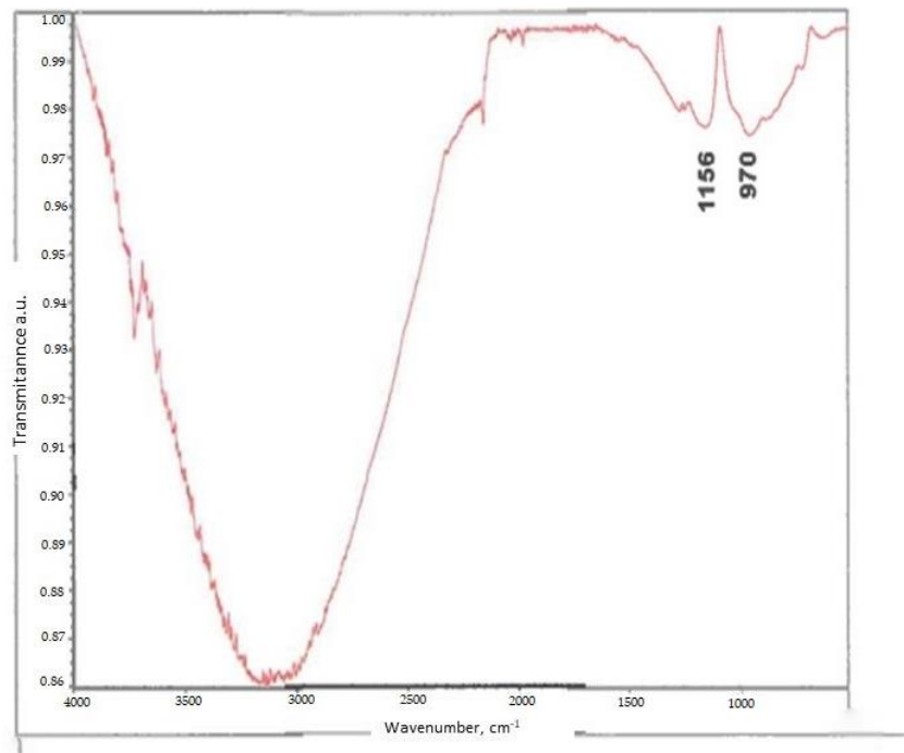
a) Figure S3. ATR-FTIR spectra of: a) SWCNT b) SWCNT-OH.
