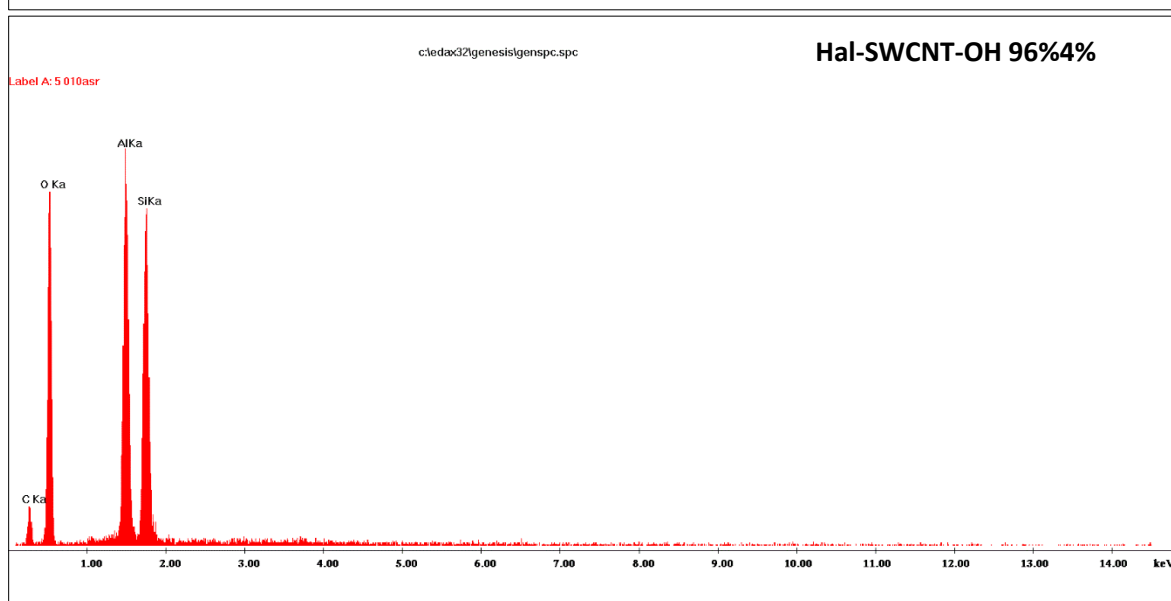
Figure S2. EDX results of Hal-CNT composites
