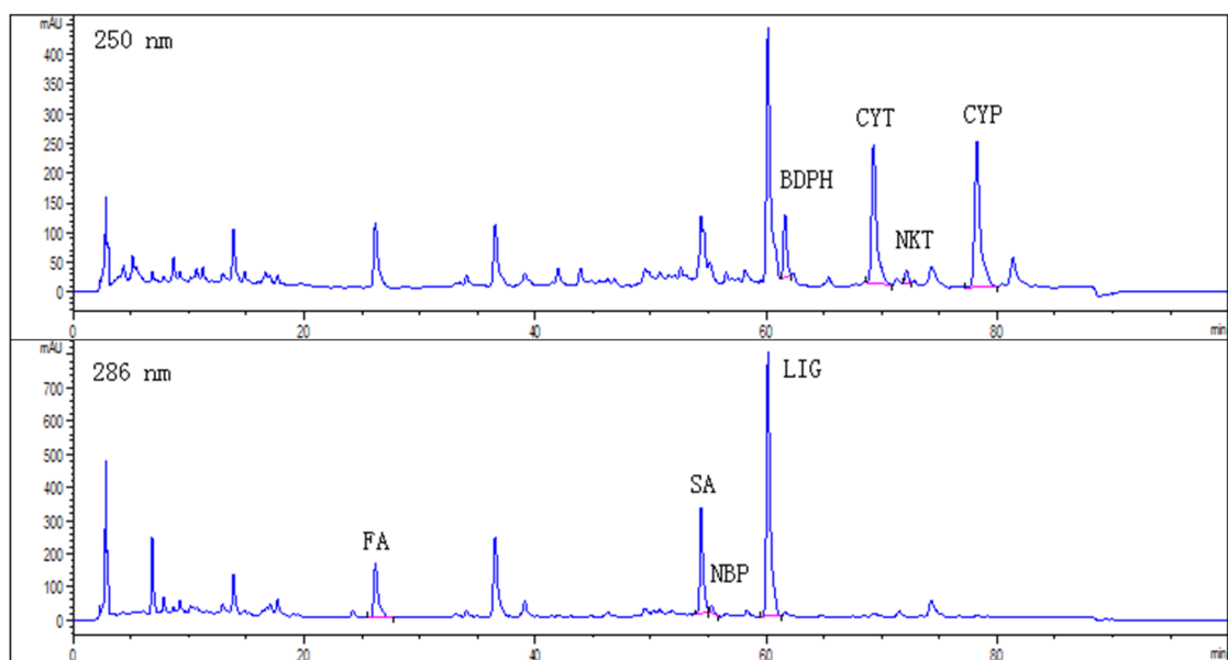
Figure S1. The HPLC chromatograms of CRCR extract solution.
