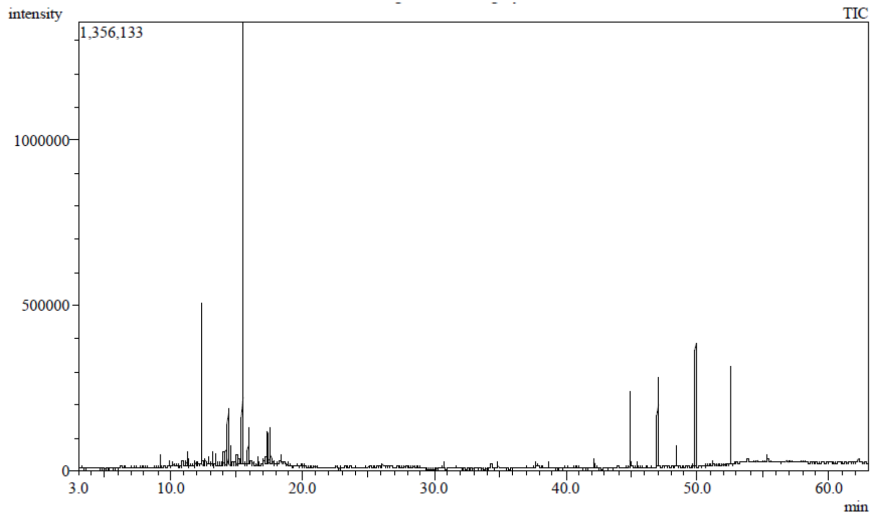
Figure 2: Gas chromatography chromatogram of Cassia javanica flowers volatile oils
