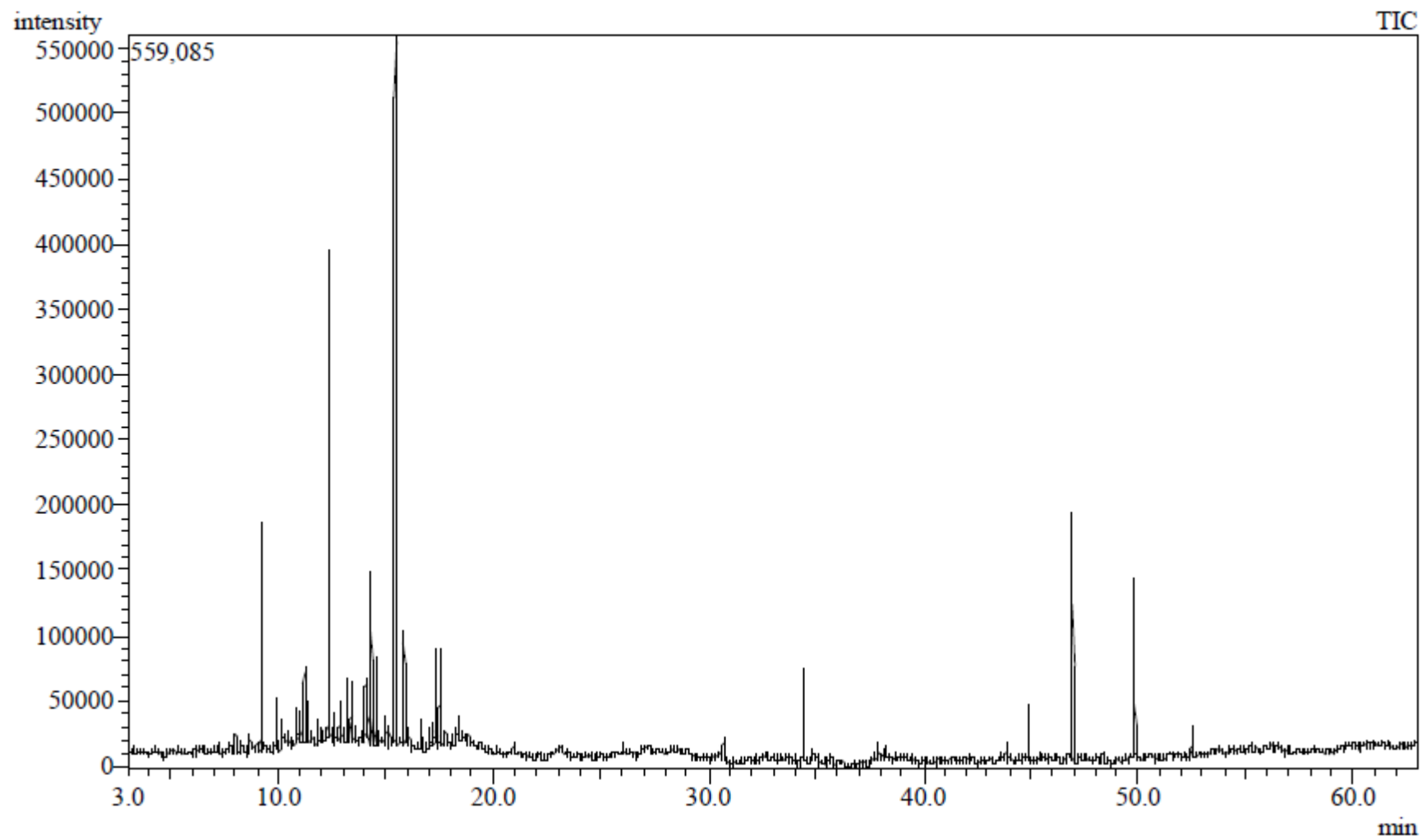
Figure 1 Gas chromatography chromatogram of Tecoma stans flowers volatile oils
