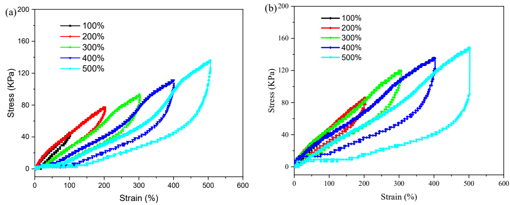
Figure S1 Hysteresis and self-recovery properties of P(AAc-co-AM)/PVA DN hydrogels at room temperature: (a) cyclic tensile loading-unloading curves under different strains at certain resting time (5min) between two successive measurements; (b) cyclic tensile loading-unloading curves under different strains at certain resting time (30min) between two successive measurements
