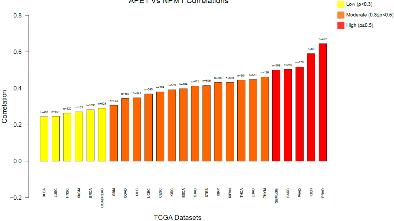
APE1 Vs NPM1 Correlations
