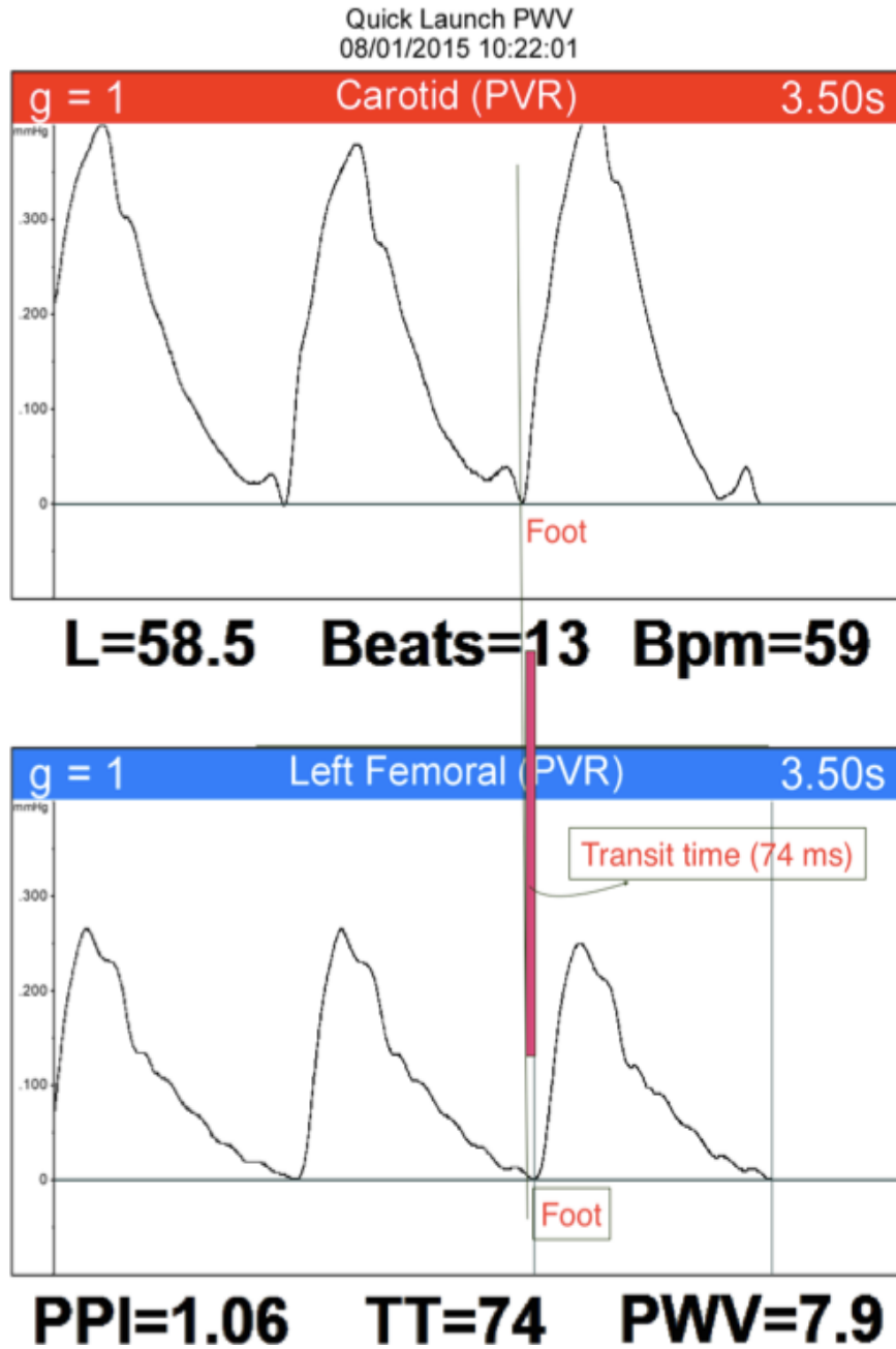
Supplementary Figure 1. Method for calculating the transit time (TT) used to derive carotid-femoral PWV, using the ‘foot-to-foot’ using the Vicorder device.
