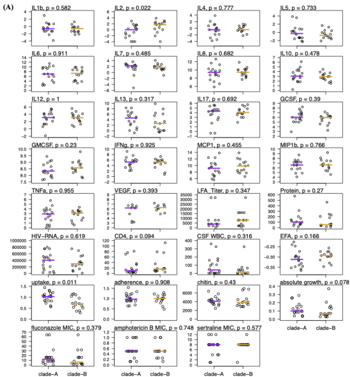
Figure S1. Clade-specific differences in phenotype. Bar indicates median value.
