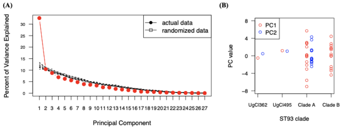
Figure S2. PCA analysis. A) Each dashed line represents one of 20 randomized trials. B) There was no association between PC1 or PC2 and clade.
