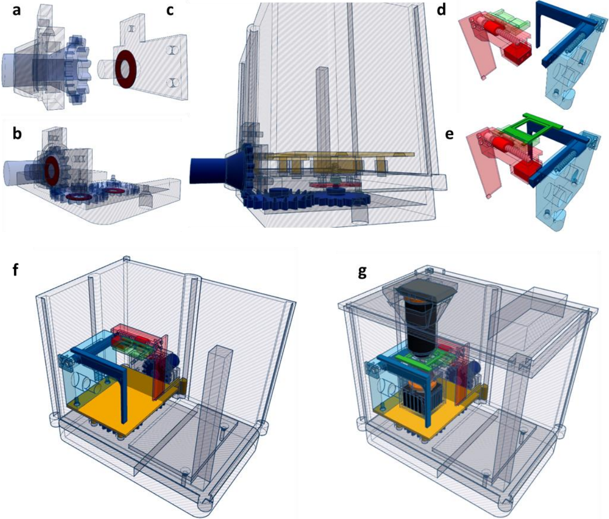
Supplementary Figure S4: Components of mobile microscope
