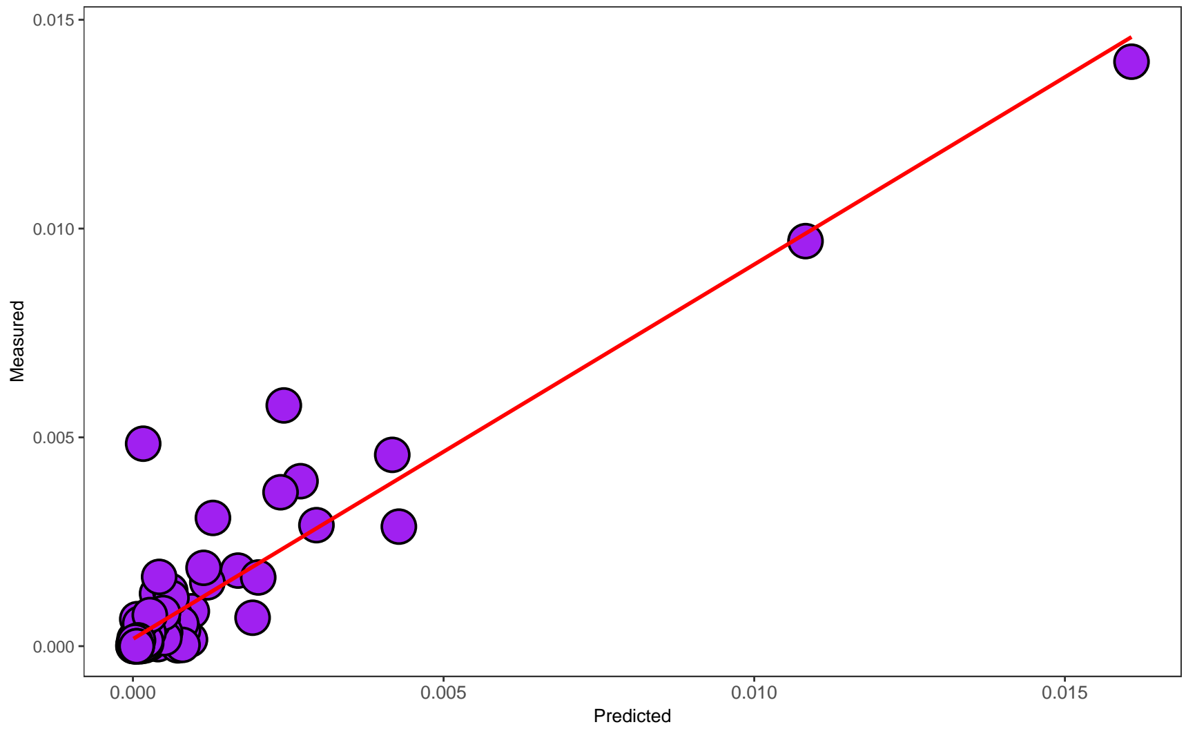
UMCGIBD00645_UC: Spearman 0.78
