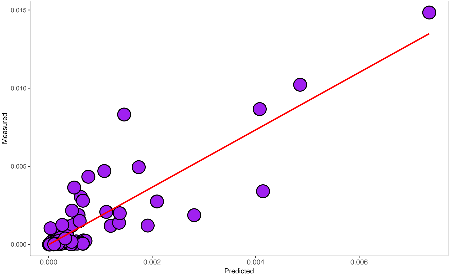
LLDeep_0034_HC: Spearman 0.75
