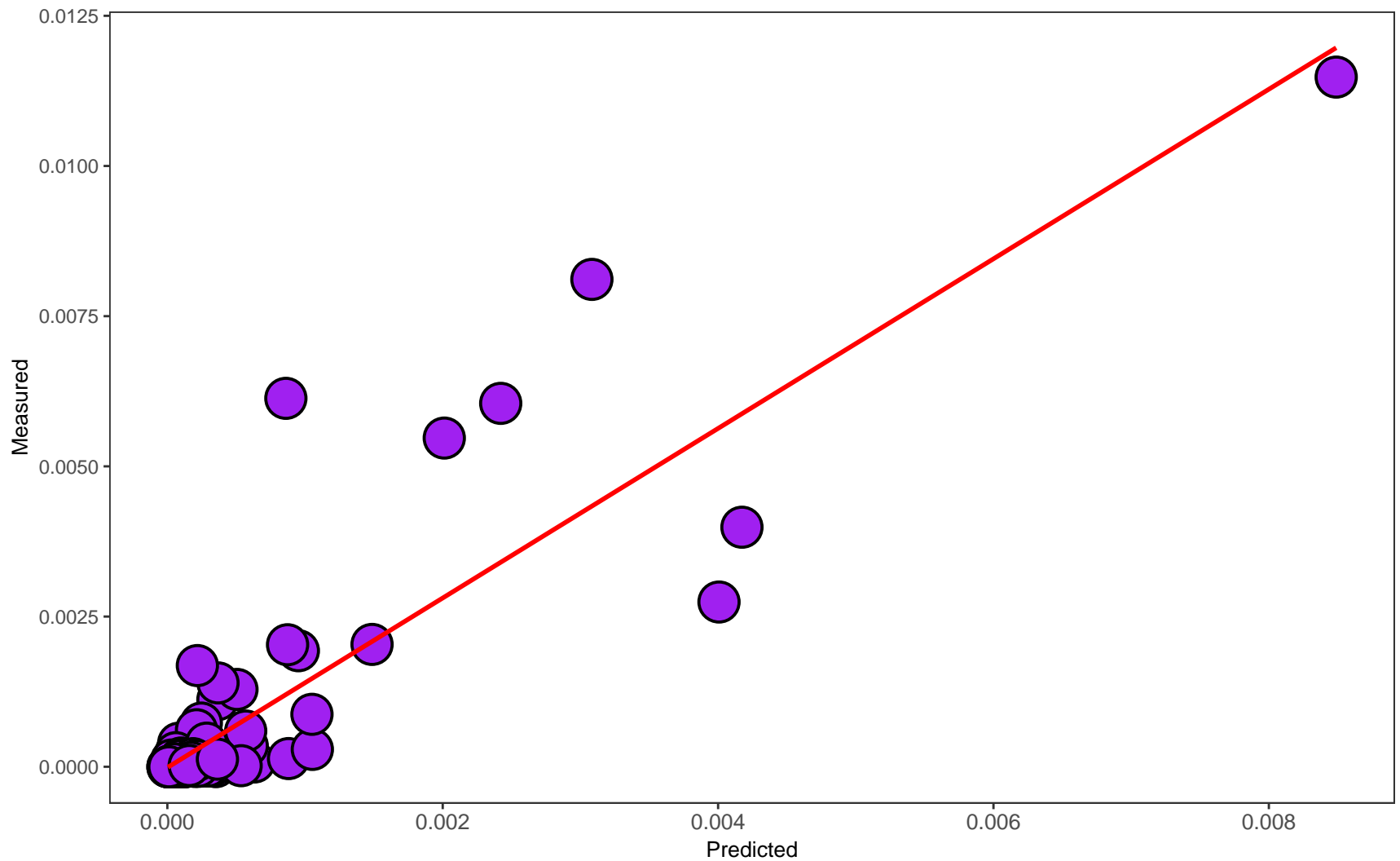
LLDeep_0033_HC: Spearman 0.73
