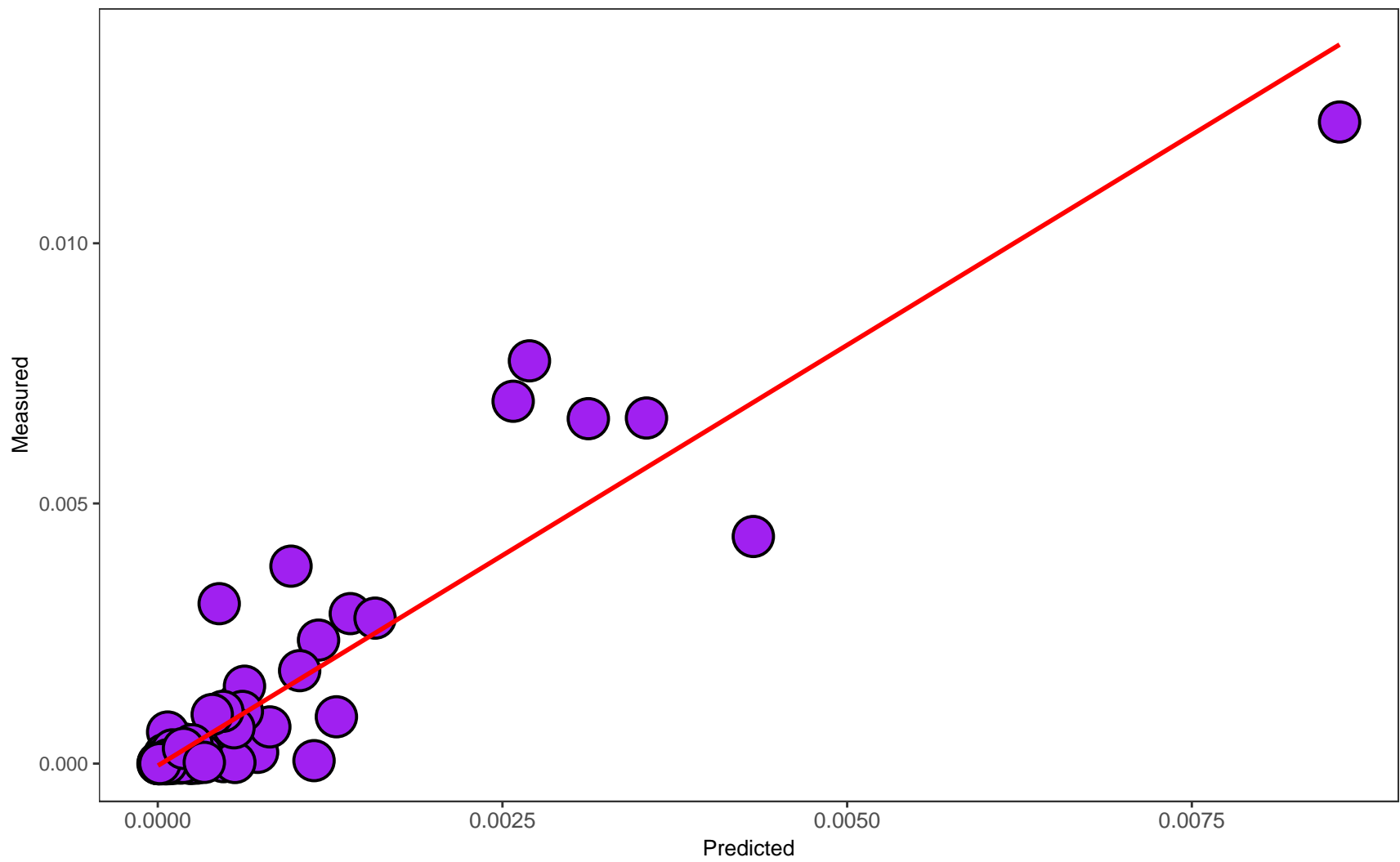
LLDeep_0021_HC: Spearman 0.77
