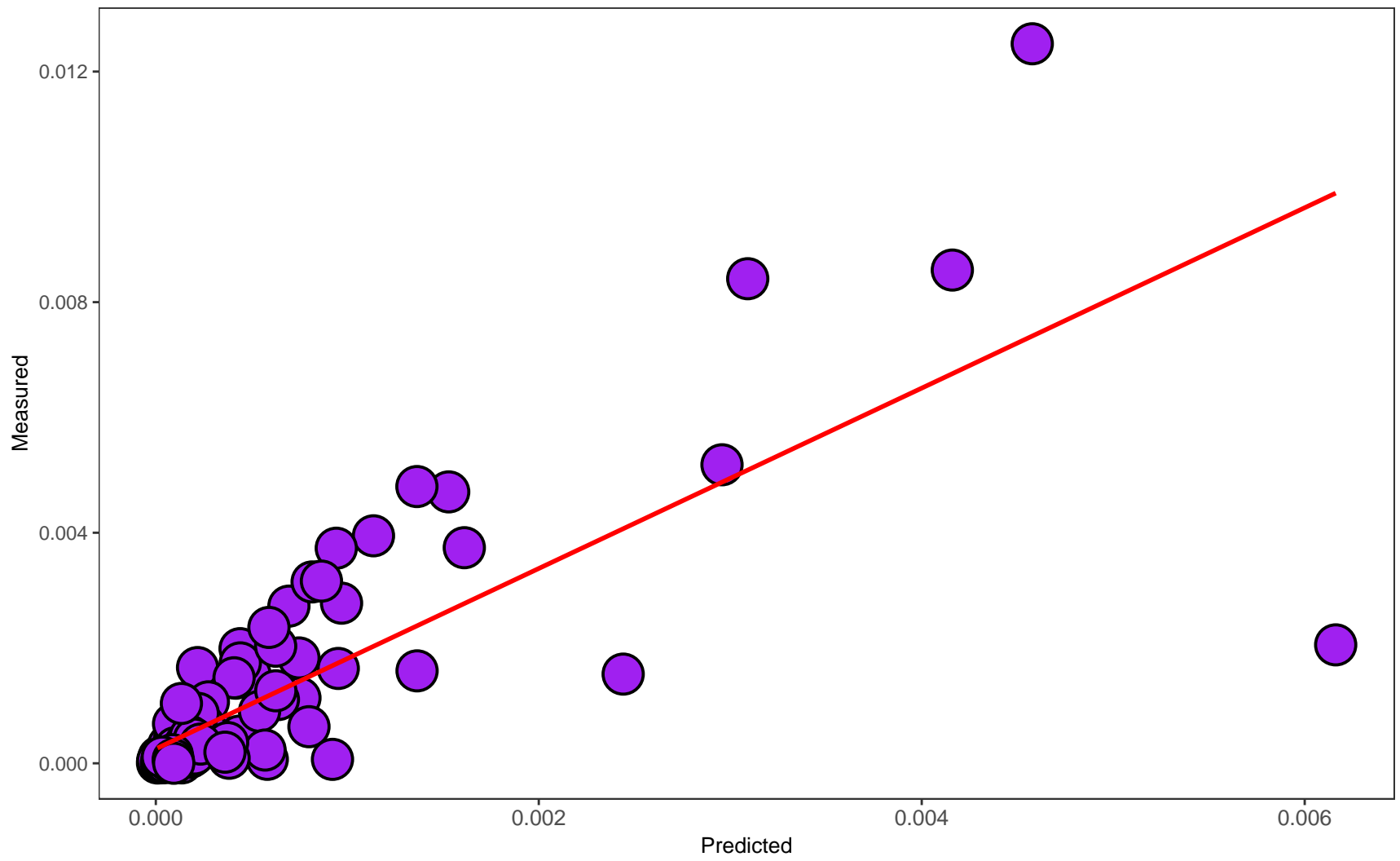
UMCGIBD00238_CD: Spearman 0.83
