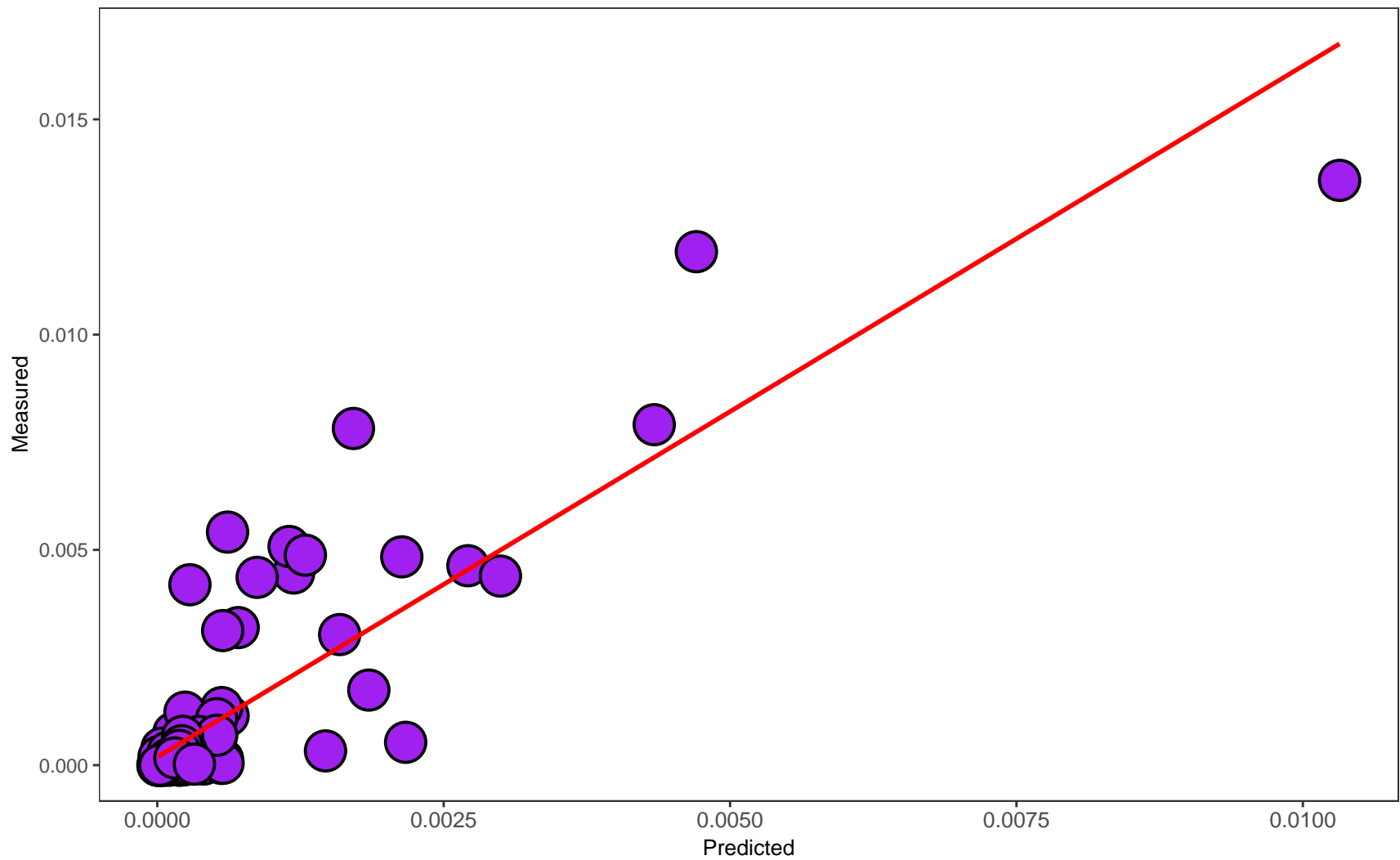
LLDeep_0022_HC: Spearman 0.75
