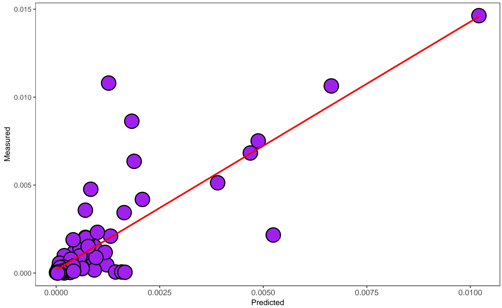
UMCGIBD00077_CD: Spearman 0.77
