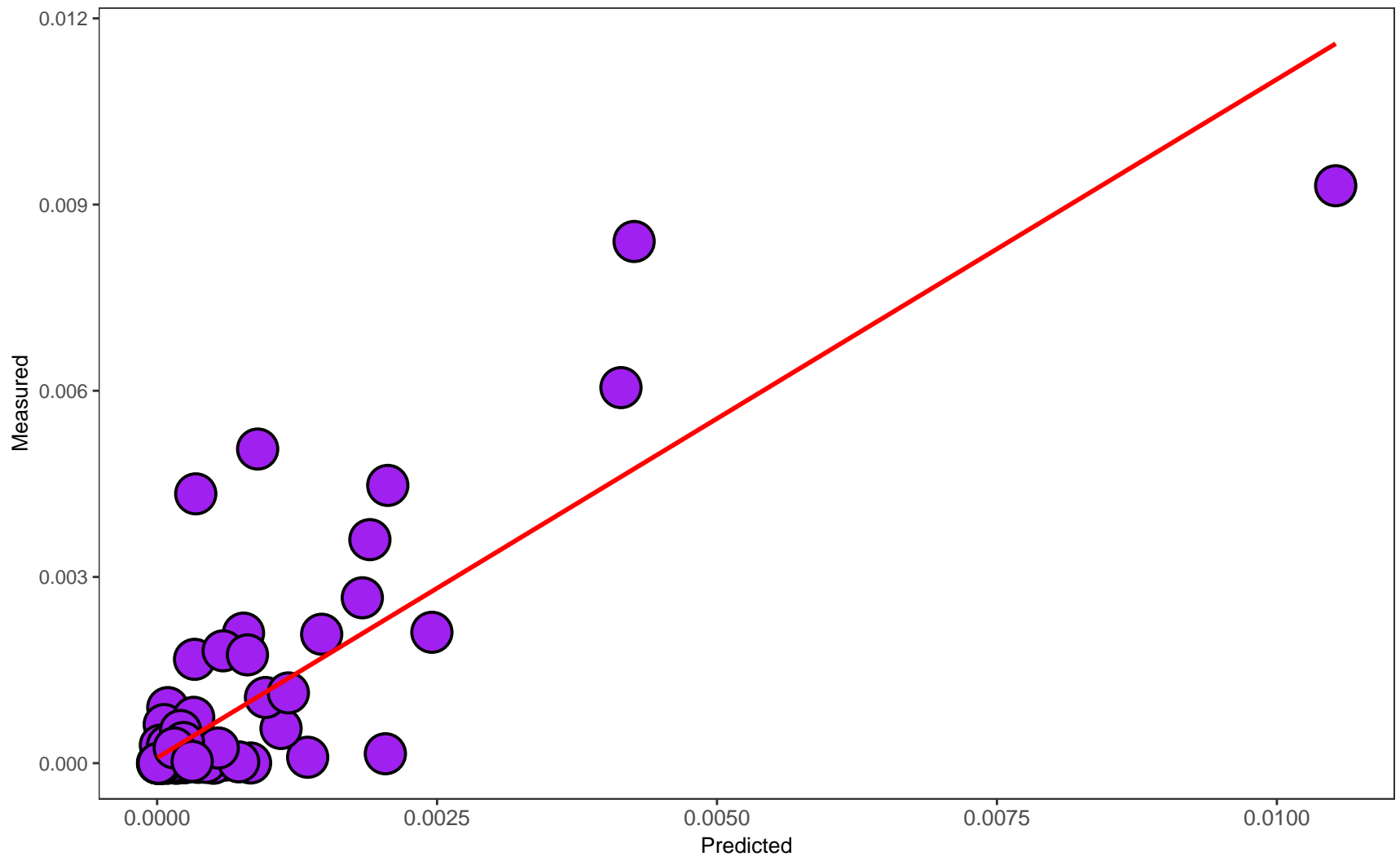
LLDeep_0037_HC: Spearman 0.67
