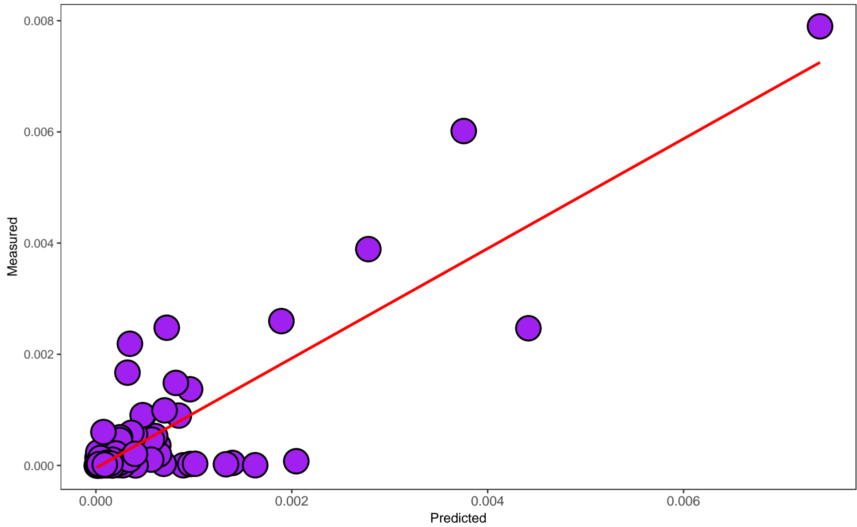
UMCGIBD00053_UC: Spearman 0.49
