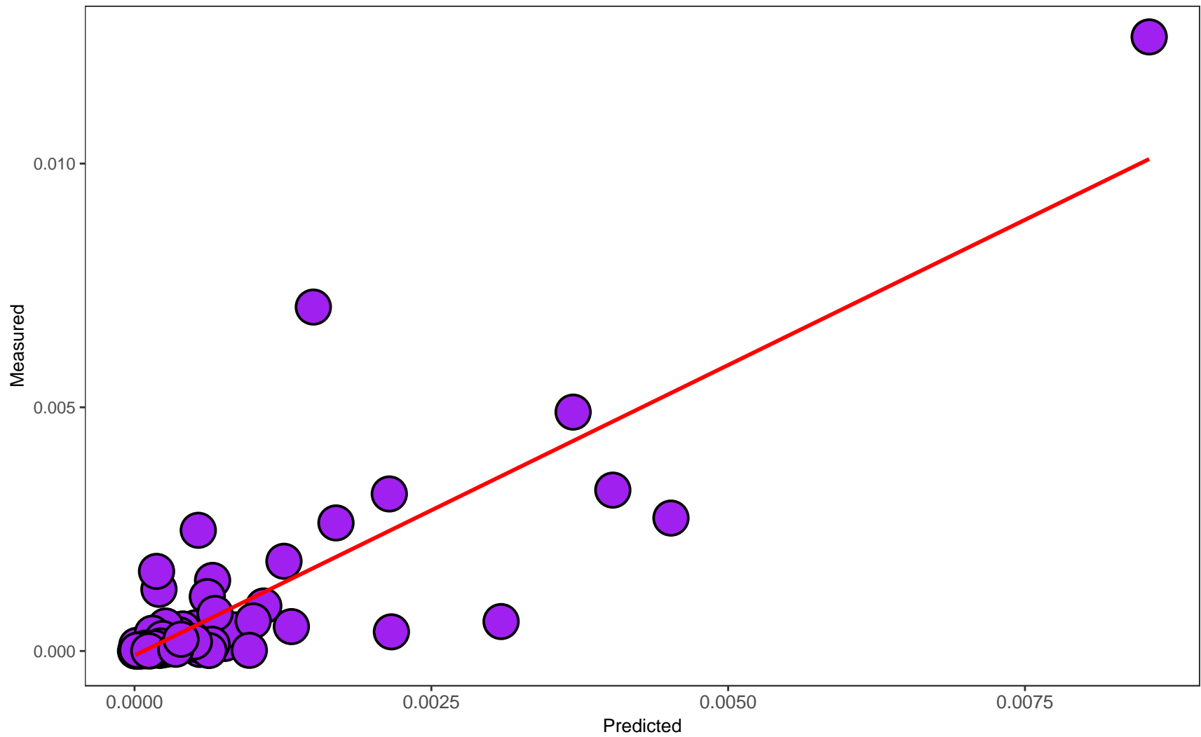
UMCGIBD00412_UC: Spearman 0.8
