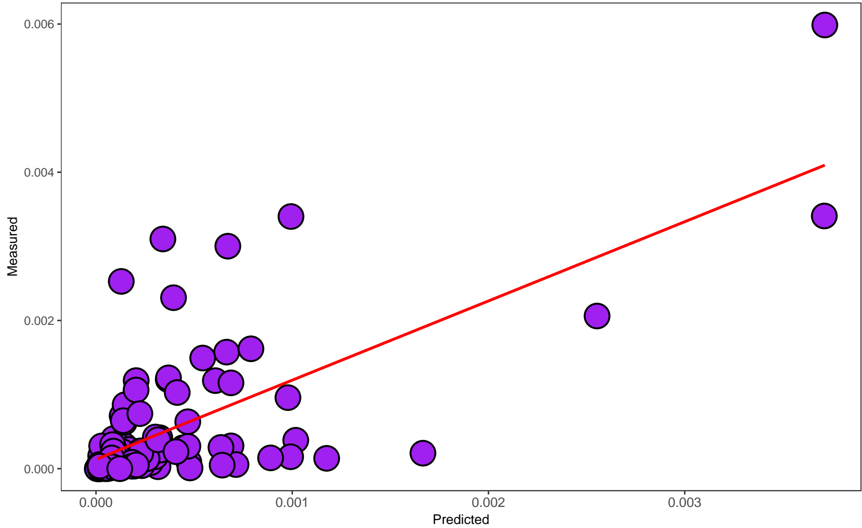
UMCGIBD00250_UC: Spearman 0.64
