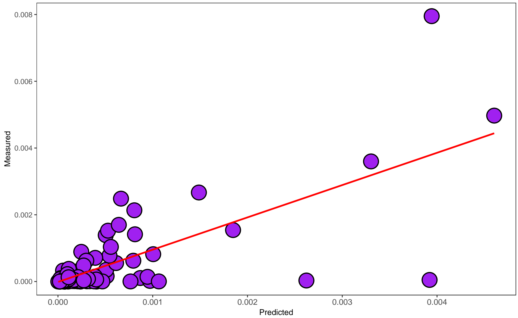
UMCGIBD00613_UC: Spearman 0.55
