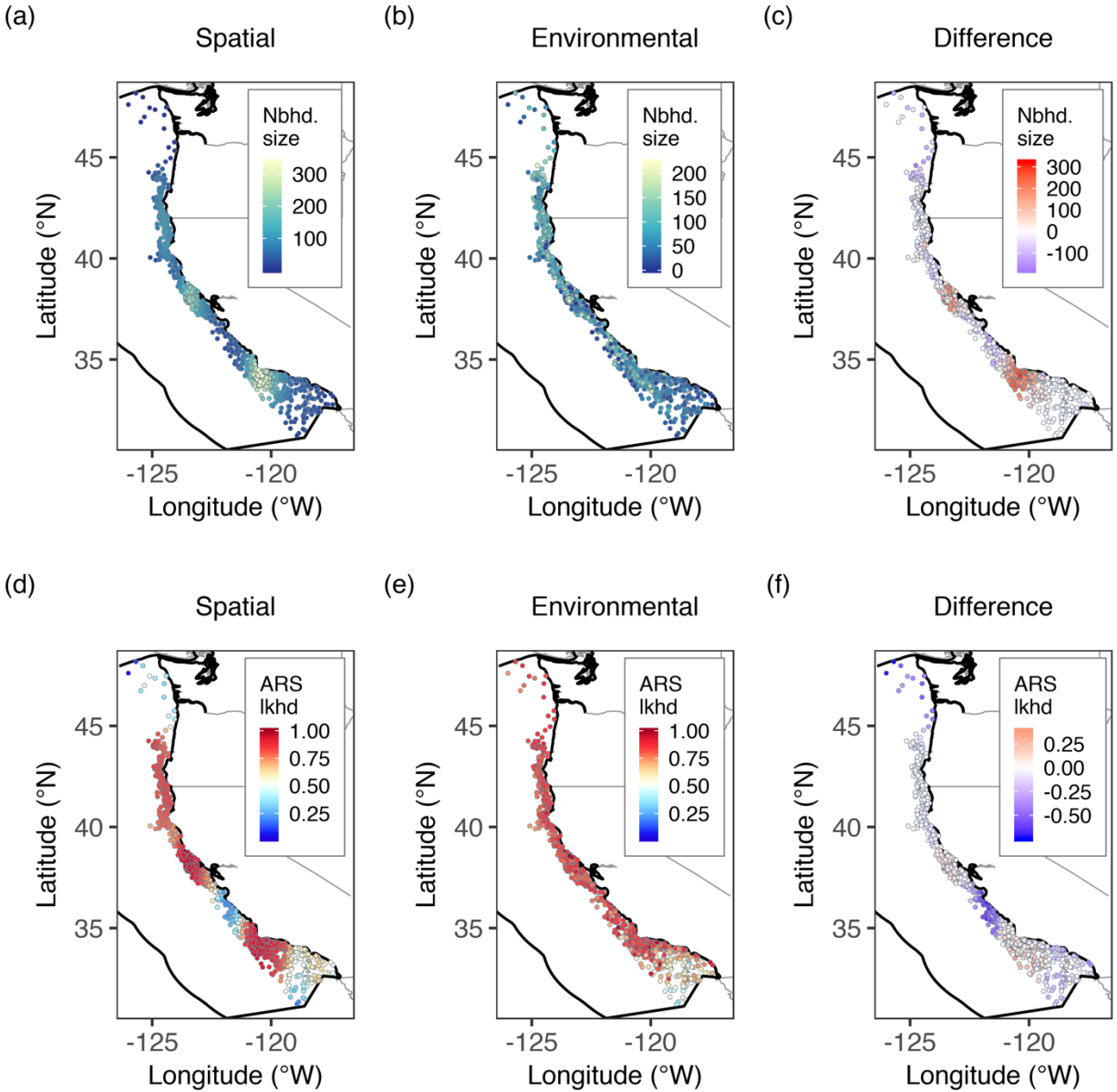
Additional file 8: Figure S8. Maps of neighborhood size (a-c) and likelihood of ARS (d-f) at each SSSM location for NPMR models based on spatial coordinates (first column), environmental predictors (second column), and the difference between the two (third column). Polygon with thick black outline is the EEZ boundary.
