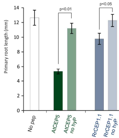
Figure S3. Comparison of activity of RrCEP1.1 and AtCEP5 with and without hydroxyprolines. Substituting canonical hydroxyprolines in positions 4 and 11 with proline markedly reduced the magnitude of host response for both AtCEP5 and RrCEP1.1 (Student's T-test, n=36-40, error bars indicate standard error of the mean).
