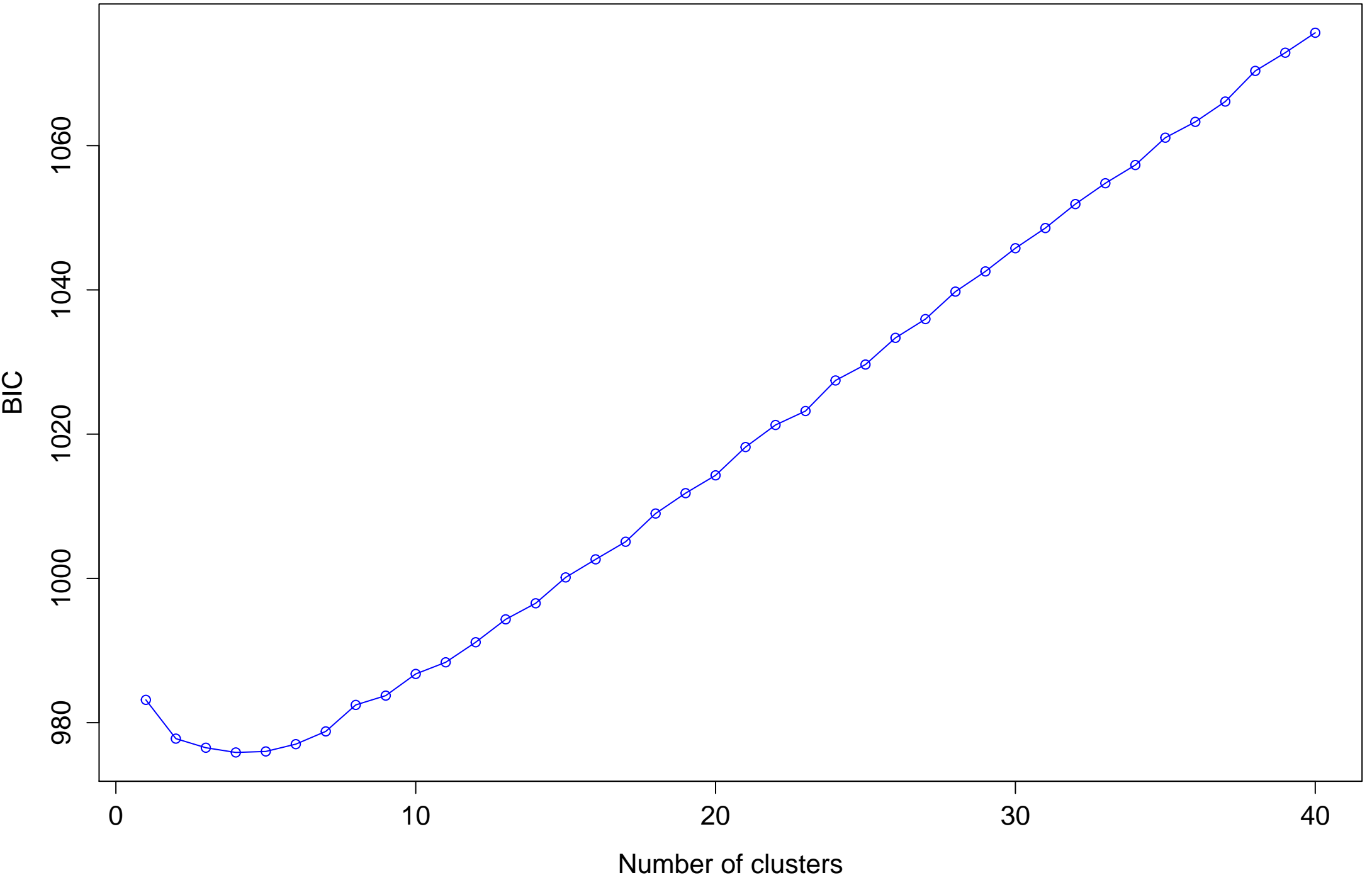
Value of BIC versus number of clusters
