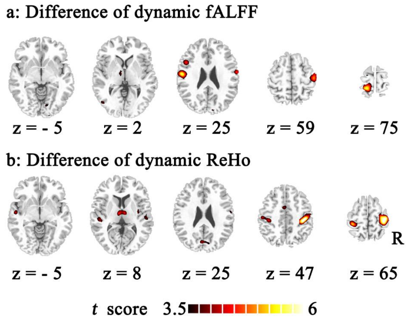
SFigure 1: Group difference of temporal variability of the dynamic fALFF and ReHo. Temporal variability of the dynamic fALFF and ReHo between schizophrenic and healthy subjects were identified using two-sample t tests. The significance level was set P_{FDR} < 0.05 . (a) the increased dynamic fALFF in schizophrenic subjects compared to healthy controls. (b) the enhanced dynamic ReHo in patients with schizophrenia.
