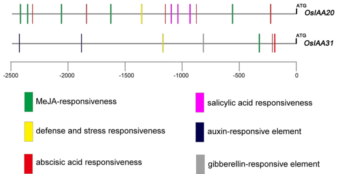
Fig. S1 The cis -element in the promoters of OsIAA20 and OsIAA31 . The 2.5 kb promoter sequence of OsIAA20 and OsIAA31 were analysed by PLANTCARE program. The different colours indicated the different binding element.
