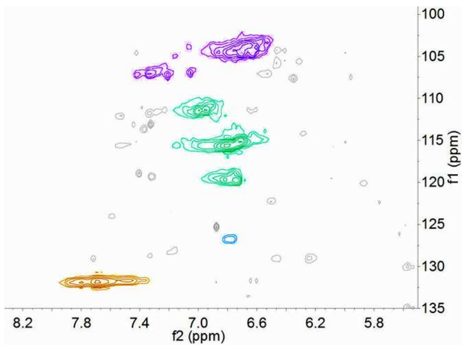
Figure S2 2D HSQC NMR of aromatic region of MWL.
