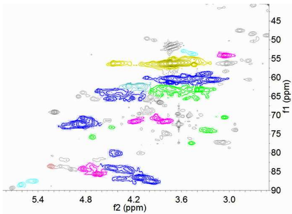
Figure S1 2D HSQC NMR of side chain region of MWL.
