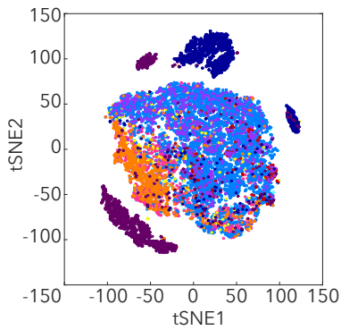
Unsupervised analysis
