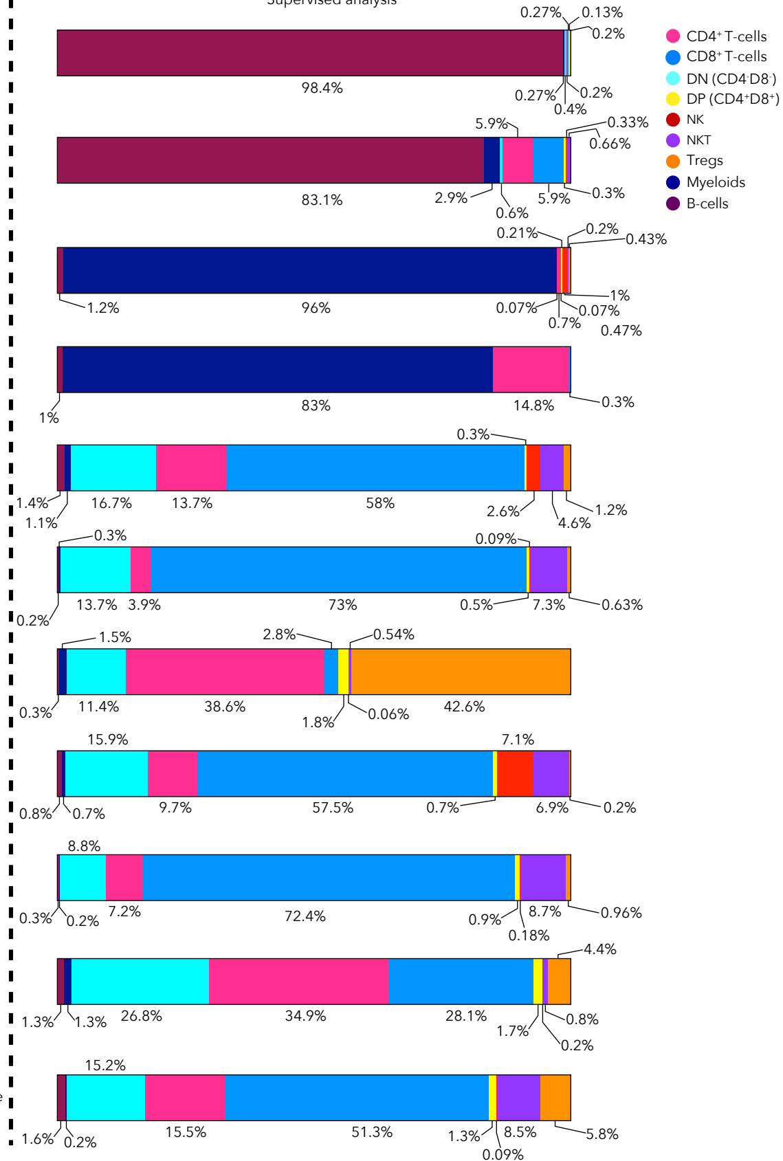
Supervised analysis
