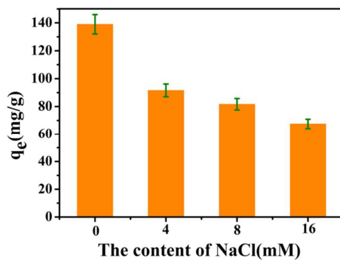
Figure S2. Effect of competitive ions on MB removal. ( C_0 [MB] = 120 mg/L, V = 100 mL, t = 12 h, pH = 9, Dos. = 50 mg, T = 30 °C)
