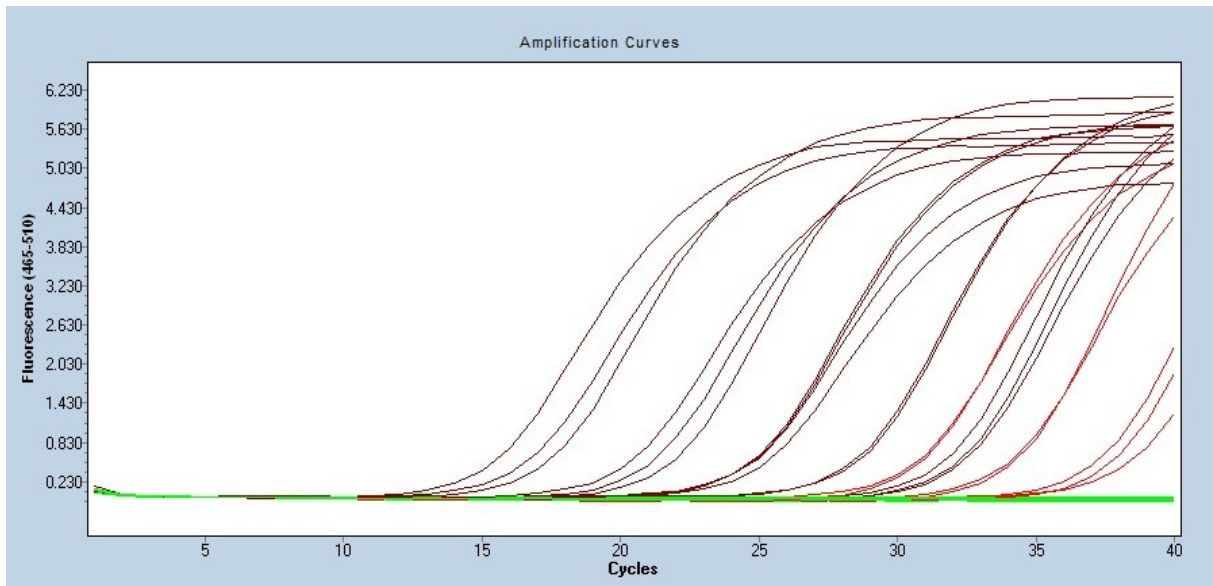
Figure S4 | Amplification curves of the TaqMan qPCR. For each DNA extract, two individual reactions were performed using 10 ng of total DNA (5 \mu l) and the amplification was examined. (A) Part 1 and (B) Part 2. >35.00 = cutoff value for the method.
