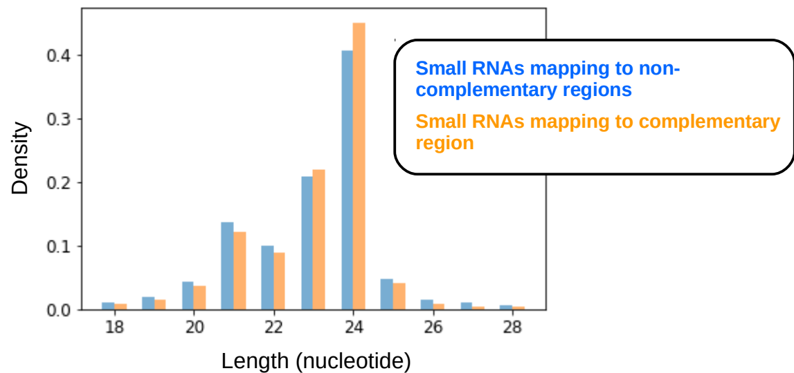
Predicted targets of trans-NATs
