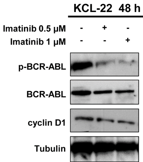
Figure S1. Levels of p-BCR-ABL, BCR-ABL and cyclin D1 in response to imatinib. Representative western blot analyses in whole cell lysates of KCL-22 cells exposed to imatinib for 48h
