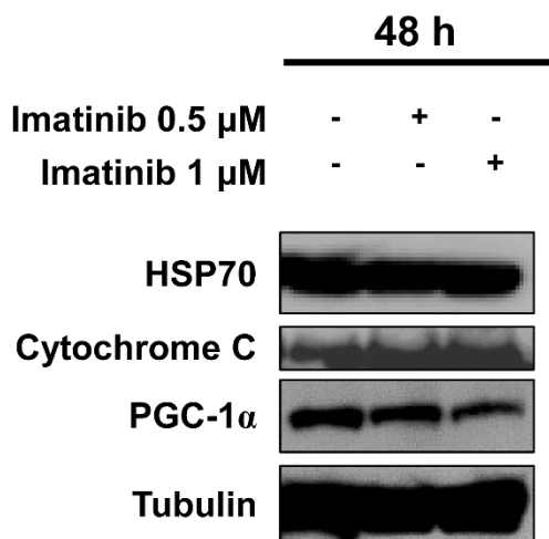
Figure S2. Levels of HSP70, cytochrome c and PGC-1 \alpha in response to imatinib. Representative western blot analyses in whole cell lysates of K562 cells exposed to imatinib for 48h
