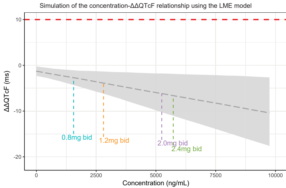
Figure S2: The vertical dashed lines indicate the geometric mean C_{max} at steady-state observed with twice daily (bid) dosing using the NEXThaler device in the Extension study. The grey area is the 90% confidence interval.
