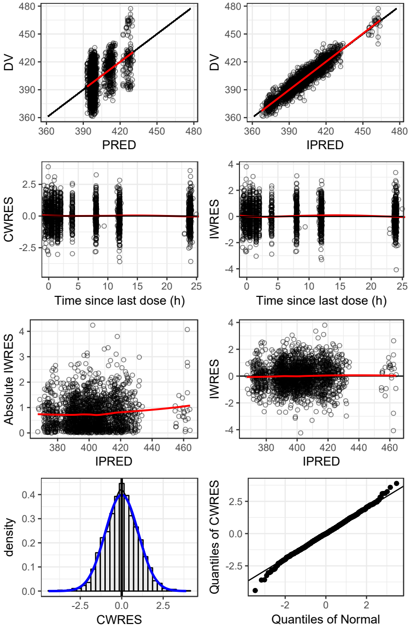
Figure S3: DV is \Delta QTcF, PRED: population predictions, IPRED: Individual predictions, CWRES: Conditional weighted residuals, IWRES: Individual weighted residuals. The clusters seen in the DV vs PRED plots are due to the covariates.
