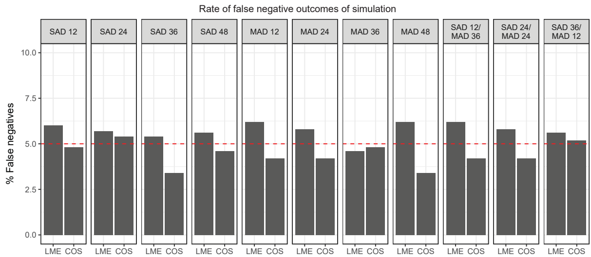
Figure S4: Rate of false negative outcomes, when the data was simulated with the Cosine model (COS) and a true slope of 0.00162 ms/pg/mL, corresponding to an increase in QTcF of 10 ms at the Cmax following twice daily dosing of 2.4 mg. The labels on each panel indicate the design (single ascending dose [SAD] or multiple ascending dosing [MAD]) and the number of subjects.
