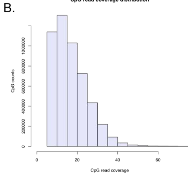
CpG read coverage distribution
