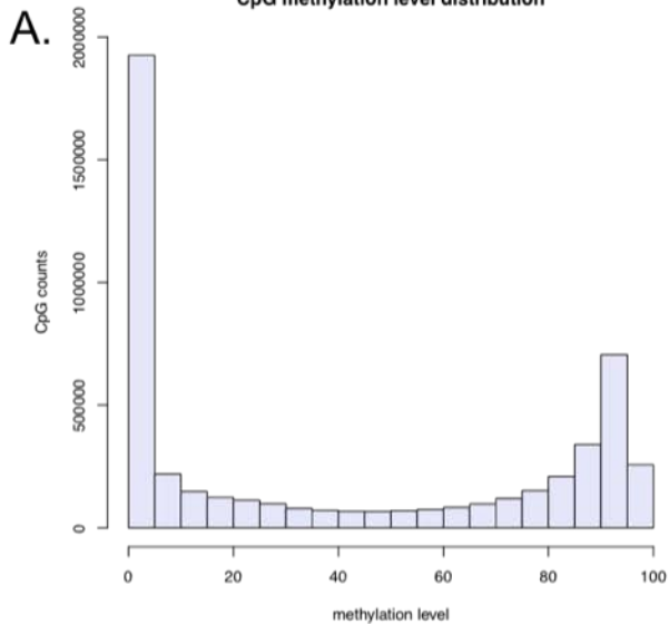
CpG methylation level distribution
