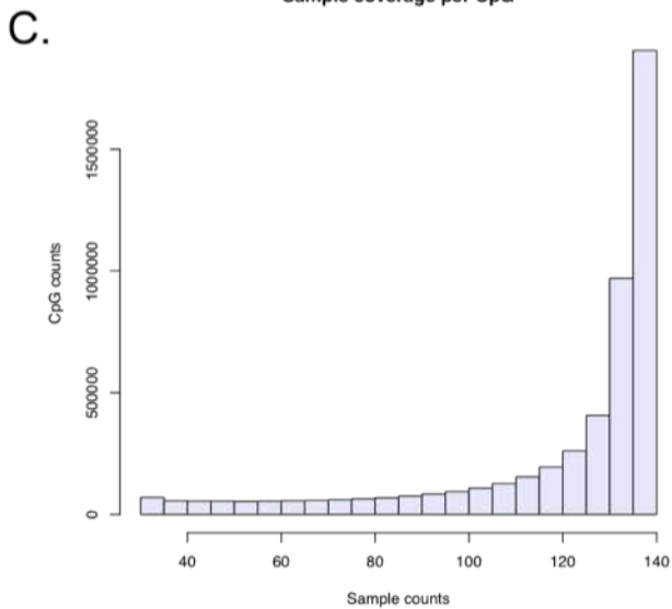
Sample coverage per CpG
