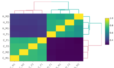
Pairwise Proportions of Shared TADs @ 50kb
