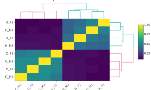
Pairwise Proportions of Shared TADs @ 500kb
