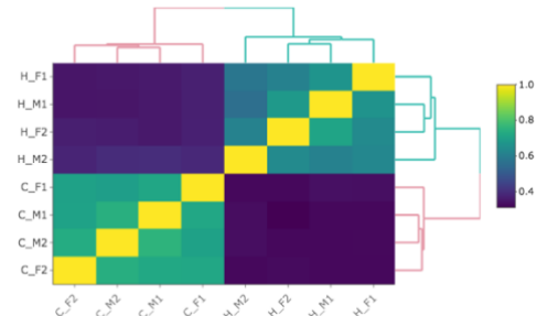
Pairwise Proportions of Shared TADs @ 100kb
