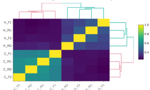
Pairwise Proportions of Shared TADs @ 250kb
