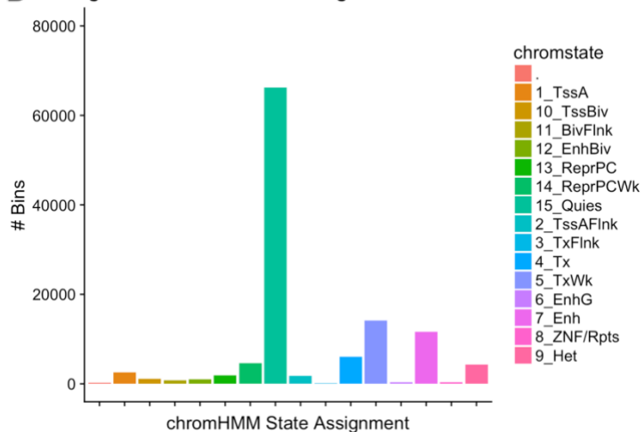
Weighted chromHMM State Assignments Distribution
