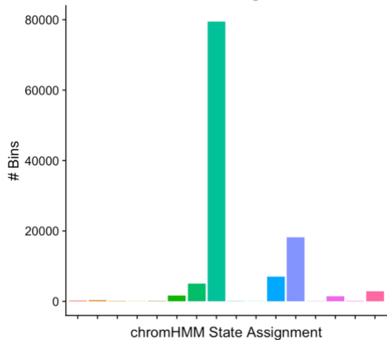
Basal chromHMM State Assignments Distribution
